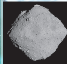
Ryugu asteroid
